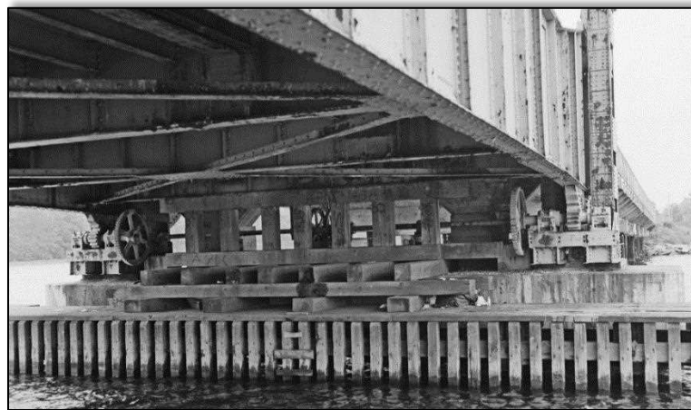
Below: Underside of lift span, showing lift gear machinery.
