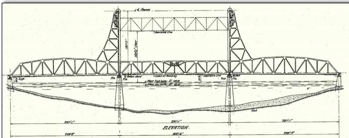
Elevation drawing from original plans prepared by J.A.L. Waddell Consulting Engineer, New York City, 1920.
