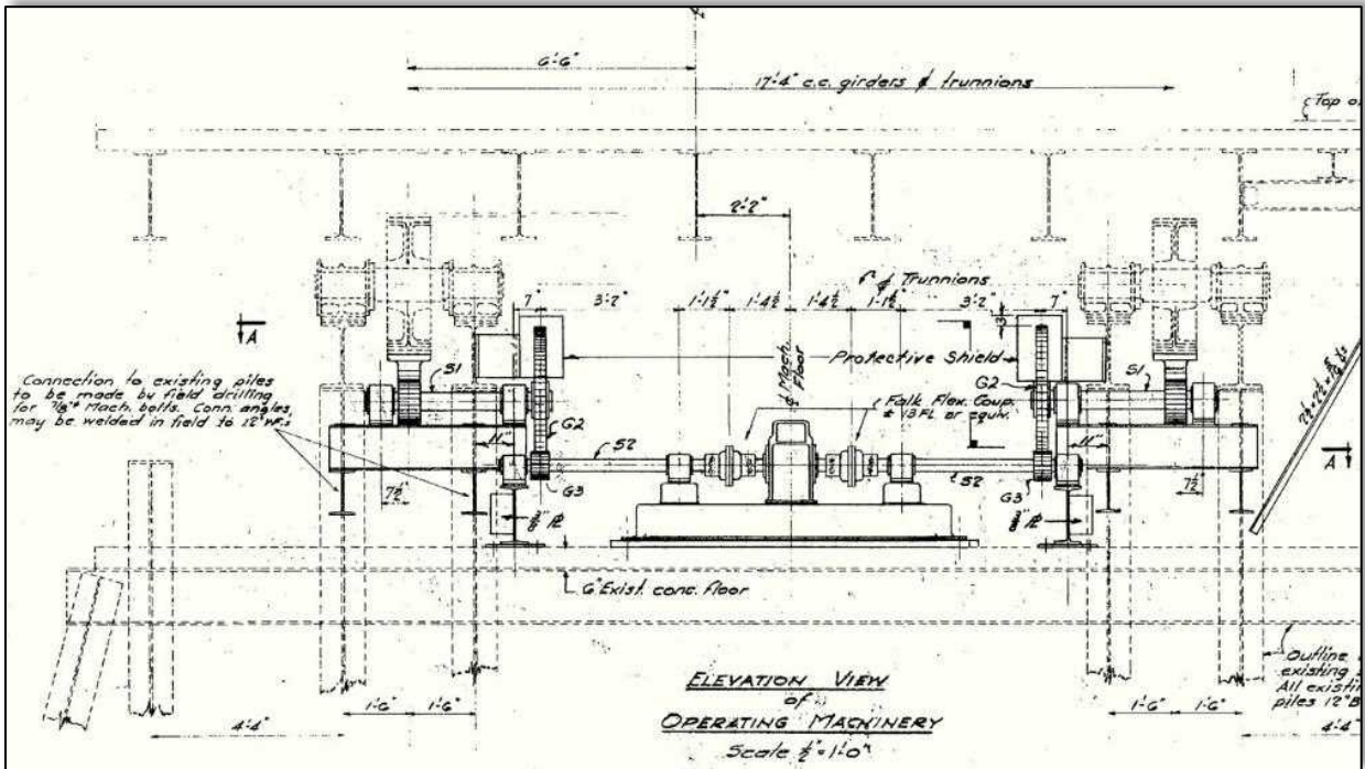
Clip from original 1962 plans for adding bascule lift operating machinery, as designed by Harold E. Langley and Robert J. Prowse. Rack and pinion gears, a reduction gear transmission and two electric motors plus associated shafting, mounts and electrical controls were installed in 1962.
